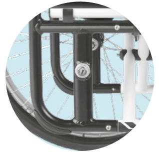
MA 114 Drive wheel adapter, permanently welded
