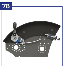
78 Locking of the integrated brake
